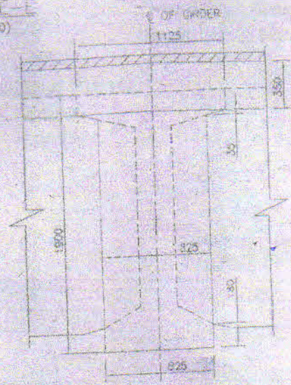
DETAIL-2 (SCALE=1/25)
