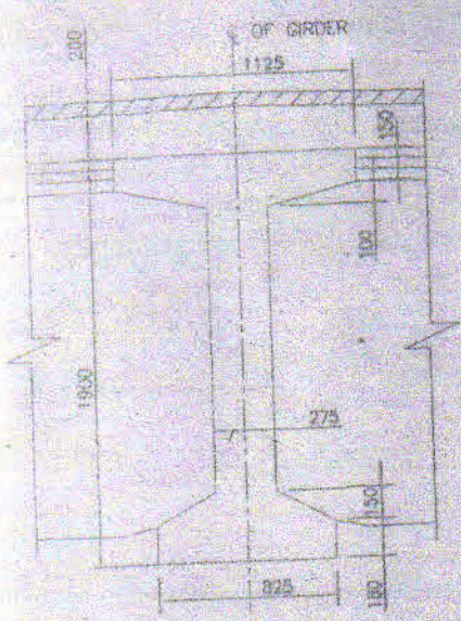
DETAIL-1 (SCALE=1/25)
