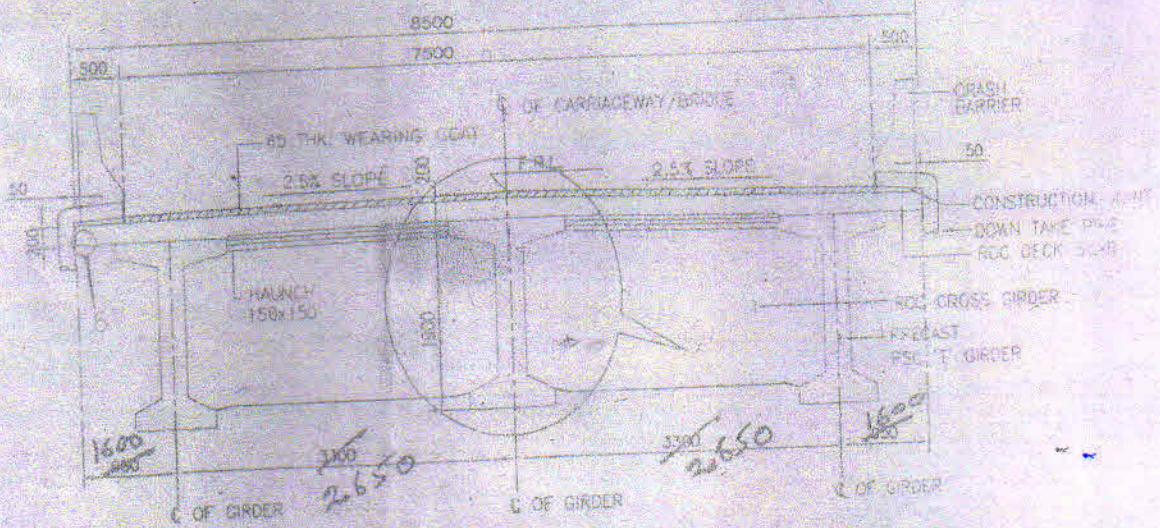
SECTION E-E (SCALE=1/30)
