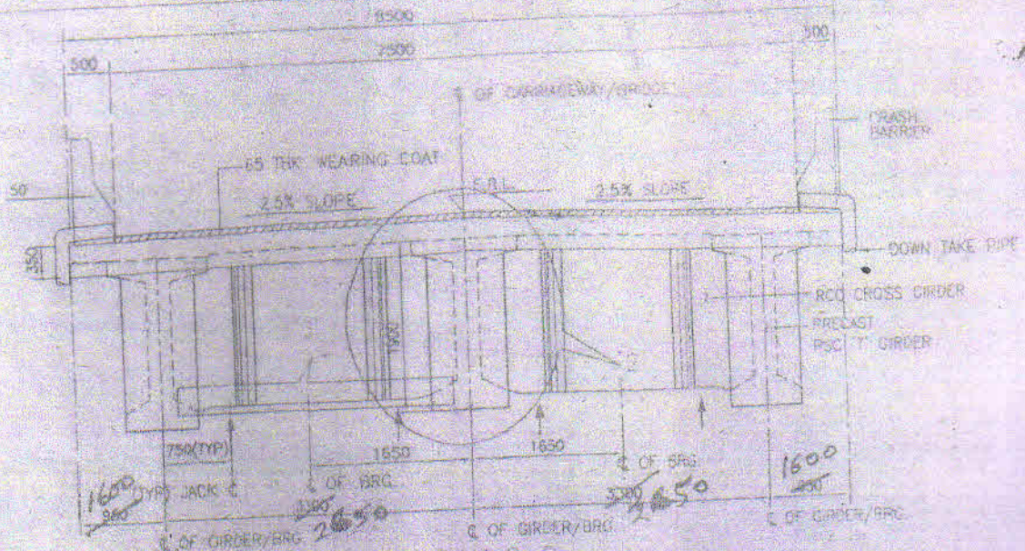
SECTION D-D (SCALE=1/30)
